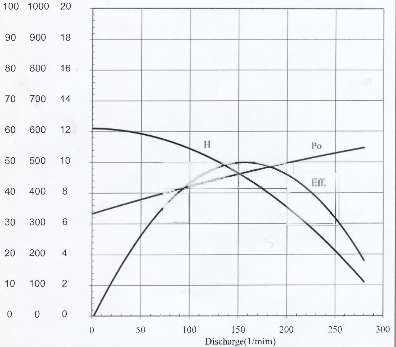
PUMP Performance Curve
